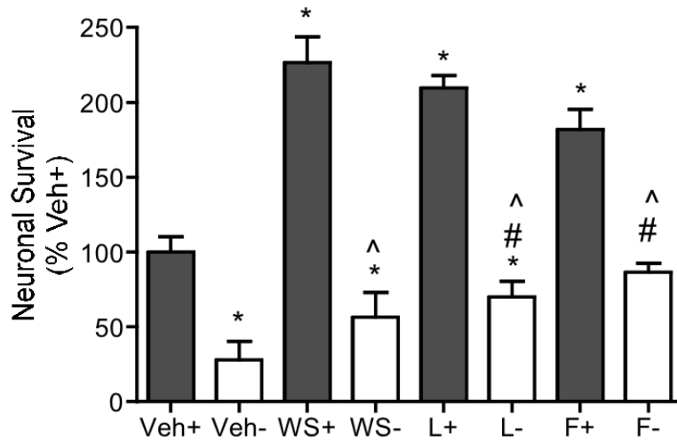
Fig. 2B. WS, withanolide A (L) and withaferin A (F) all significantly increased cell survival over that of vehicle controls (Veh+) under full nutrient conditions ( P < .0001 ). However, for the nutrient-deprived conditions (N2-), withanolide A and withaferin A, but not WS ( p = 0.065 ), significantly increased neuronal survival above that of Veh- ( P = .05 ). Determined using the lactate dehydrogenase assay
