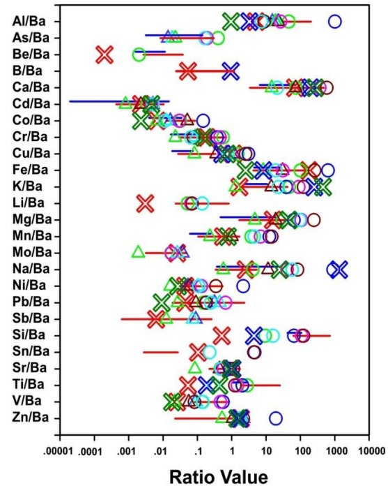
Fig. 4. Element-ratios determined for air-drop material samples are indicated by X's: Green by the Michigan Department of Environmental Quality, red by Northern Lake Service, and blue by Basic Laboratory. For comparison: Red lines and blue lines, respectively, are the measured element-ratio ranges of European [25] and American [26] coal fly ash samples, circles are element-ratios of samples of fibers (Fig. 5) found on grass as snow melted in Laona, Wisconsin (USA) on March 19, 2015, and triangles are element-ratios determined on dust collected on high-efficiency air filters operated outdoors for three month periods [13,23]
