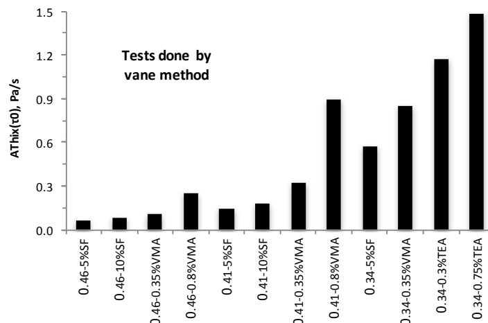
Fig. 8. Effect of mortar composition on A_{Thix}(\tau_0) measurements
