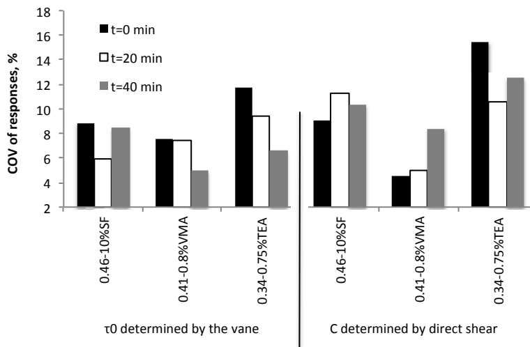
Fig. 5. COV of \tau_0 and C responses determined at different t_{rest}
